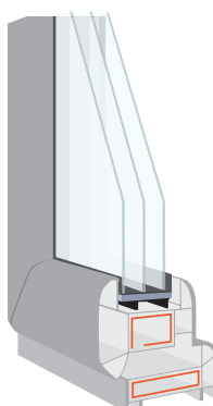
Triple Glazed
